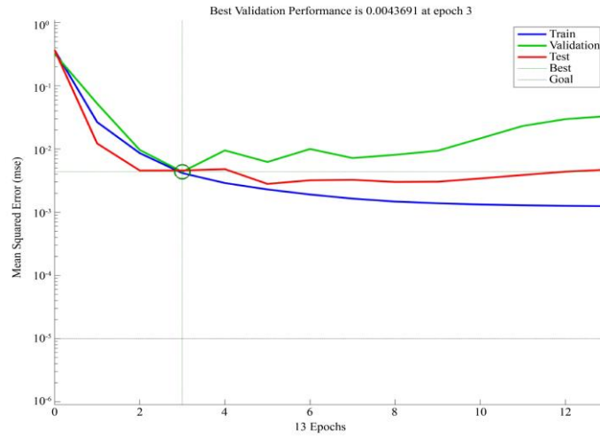
Fig. 3 The shape of the 115's network RMSE error
