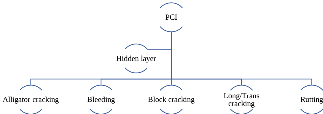
Fig. 2 The ANN network
