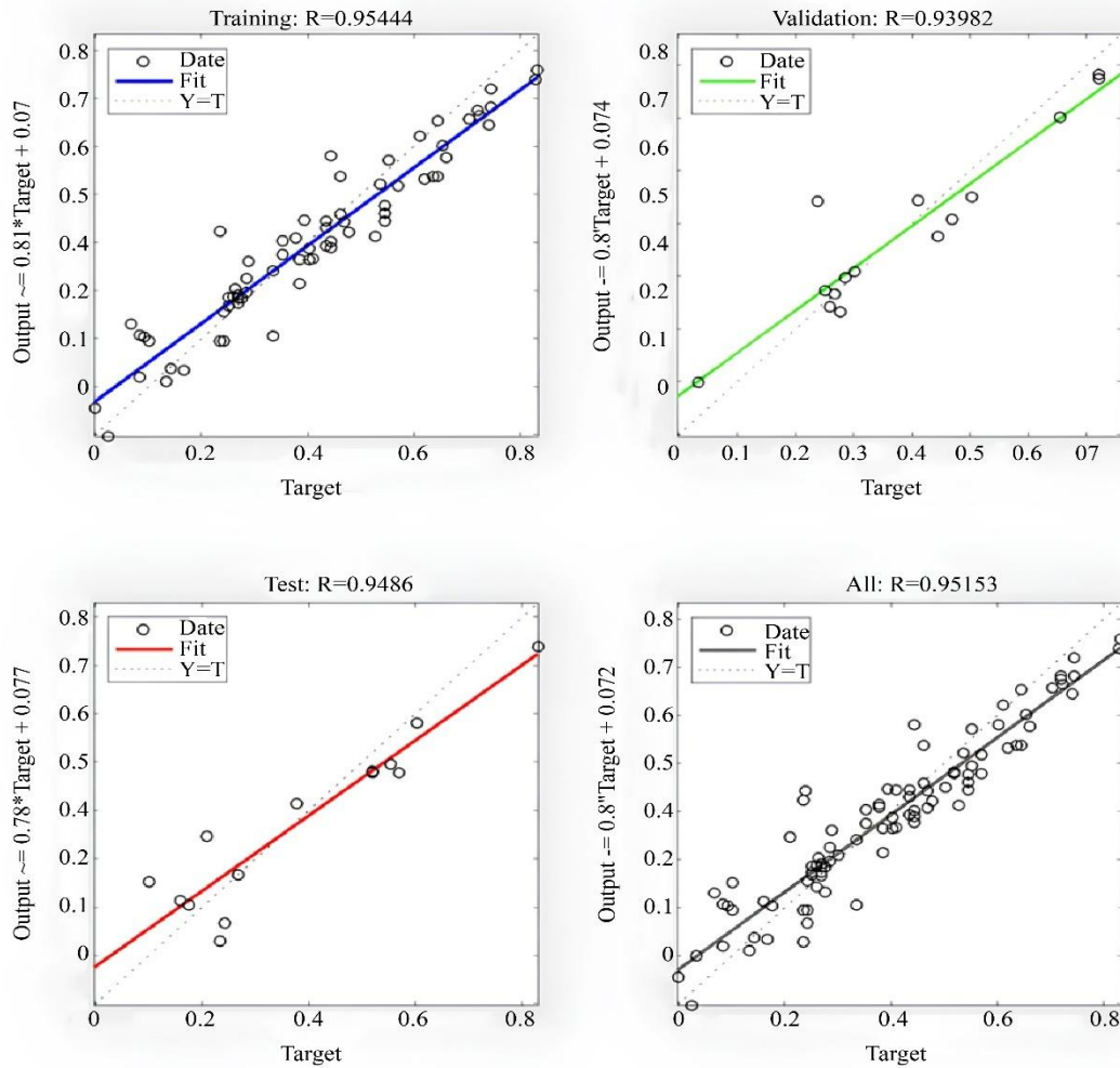
Fig. 4 The 115's network R^2 errors
